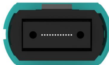
12 Fiber MTP/MPO
