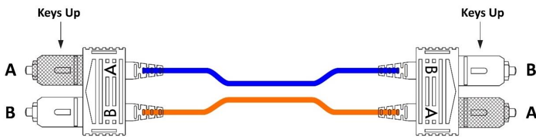
CROSSOVER POLARITY 'A' to 'B' (Nexconec Standard)
